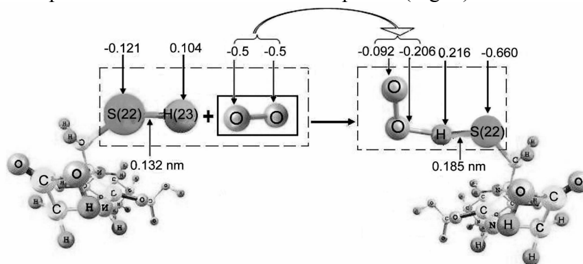
Fig. 2 - Scheme of interaction of GSH molecule with \bullet\text{OO}^- (arrows point to charges on atoms according to Lyovdin)
