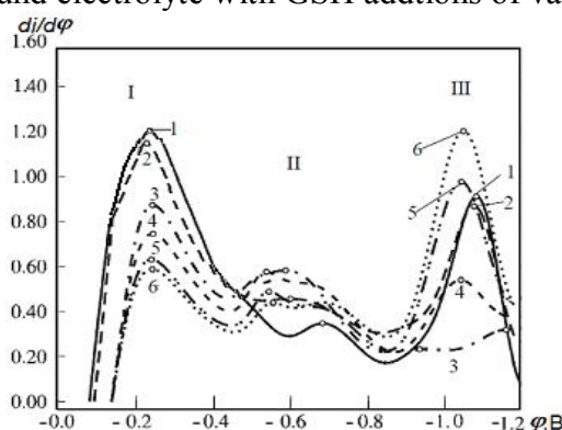
Fig. 5 - Differential volt-ampereograms of reduction of free oxygen radicals on a copper cathode against a background of 0.1 M NaCl in water (1) in the presence of various concentrations of GSH (T = 298 K): 2 - 0.24; 3 - 0.47; 4 - 0.74; 5 - 0.91; 6 - 1.1·10 3 M/ml
