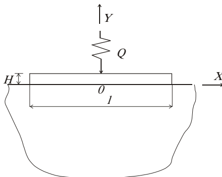
Figure 1. Calculation scheme of the concrete slab, which is deformed on the basis of the impulse load
