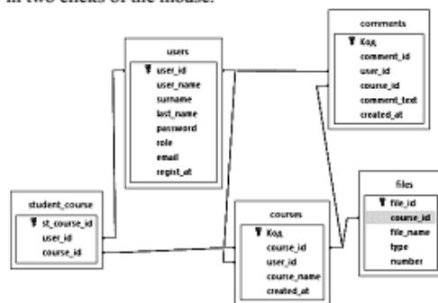
Fig. 3. Structure of the database
