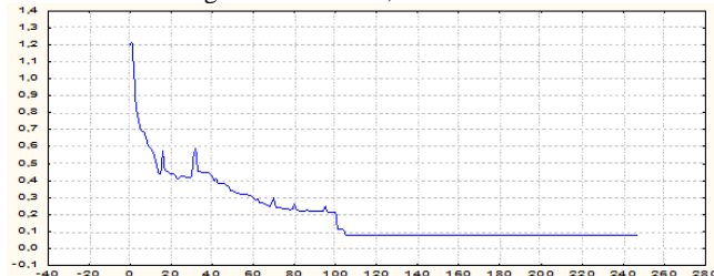
Fig.6: The training schedule on the sample fragment
