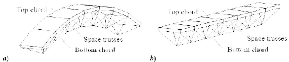
Figure 1. The steel and concrete composite cable space frame: a) arched element; b) beam element
