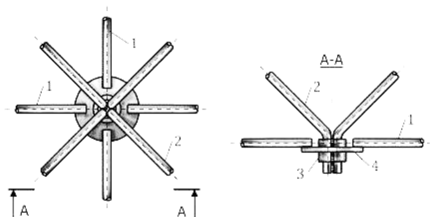
Figure 5. Welded connection (node 2): 1 – flexible rod; 2 – rod; 3 – coupling; 4 – steel round plate
