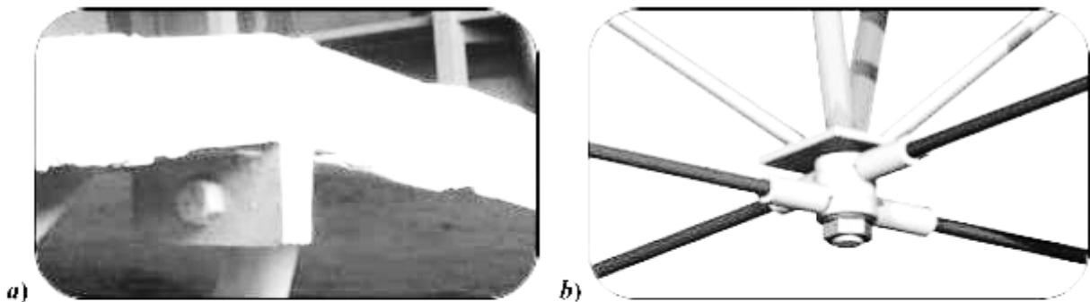
Figure 4. Bolted connections: a) node 1; b) node 2
