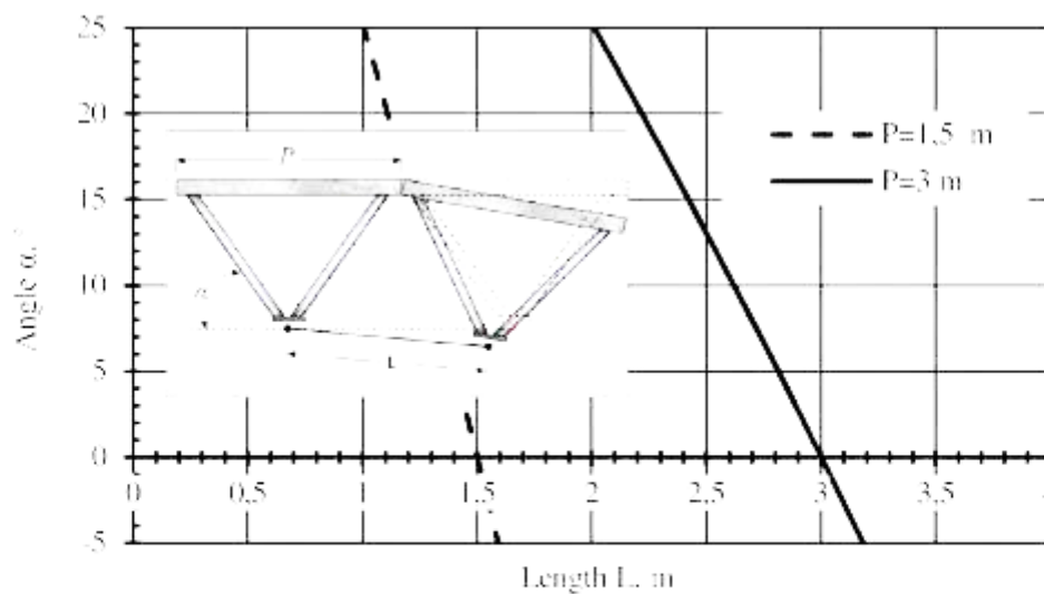
Figure 7. The length determination of the bottom chord of the steel and concrete composite cable space frame
