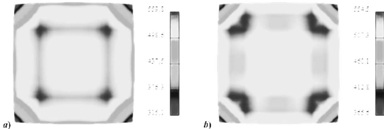
Figure 9. Plate VonMises stress (MPa):
