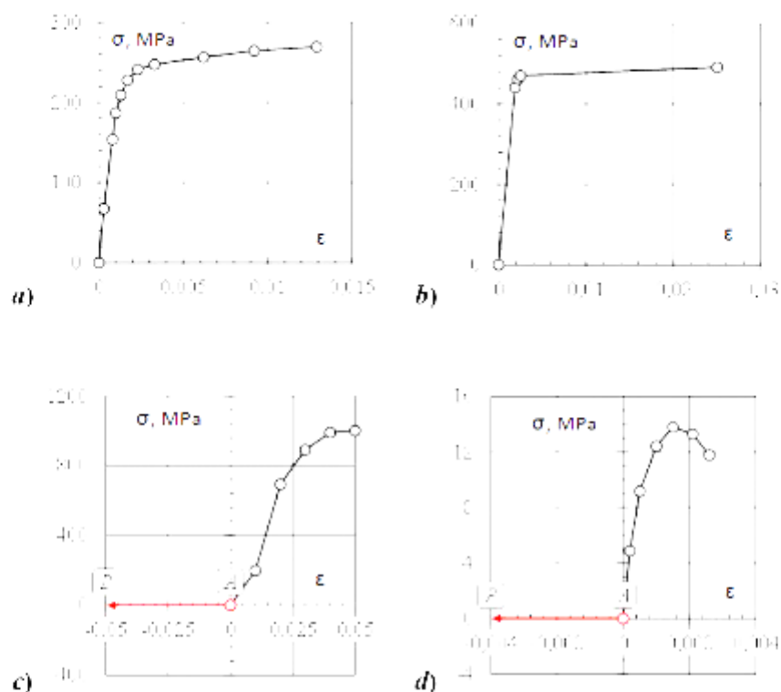
Figure 10. The stress-strain curves:
