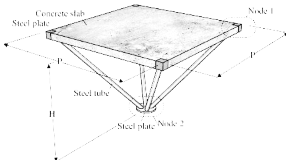
Figure 2. The steel-concrete space units of the steel and concrete composite cable space frame
