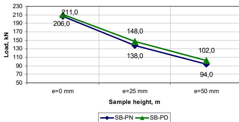
Figure 8 – Carrying capacity dependence of tested steel-reinforced concrete samples with sheet reinforcement from eccentricity at samples height h = 2,4 m
