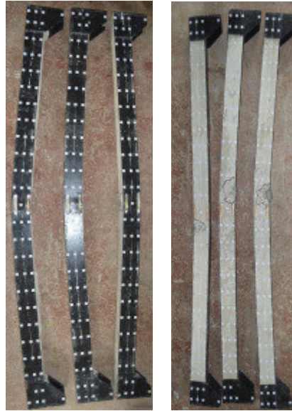
Figure 9 – The destruction of experimental steel-concrete samples with sheet reinforcement of the series SB-PD-24-1..3 and SB-PN-24-1..3 nature
