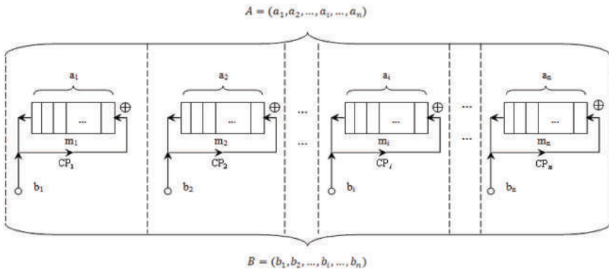
Fig. 2 – Chart of operation device of SPCIP for arbitrary MNS
