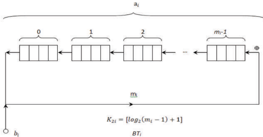
Fig. 1 – Adder in modulus m_i in MNS
